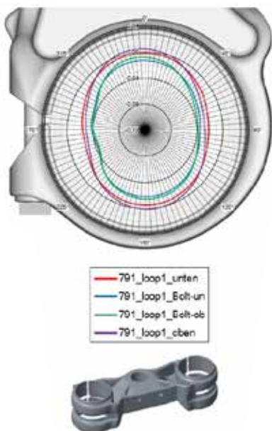
Factory Clamp
